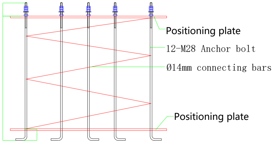
Anchor bolt positioning large sample
